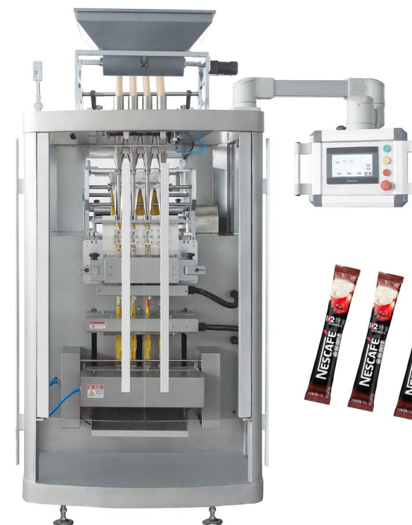
SticTop-480 Multi Lane Vertical Packing Machine
